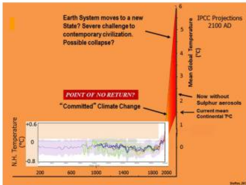
Figure 2.15: Historical and predicted global temperatures.
