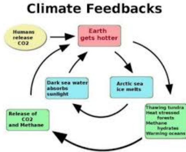
Figure 2.16: Some of the feedback loops involved in climate change.
