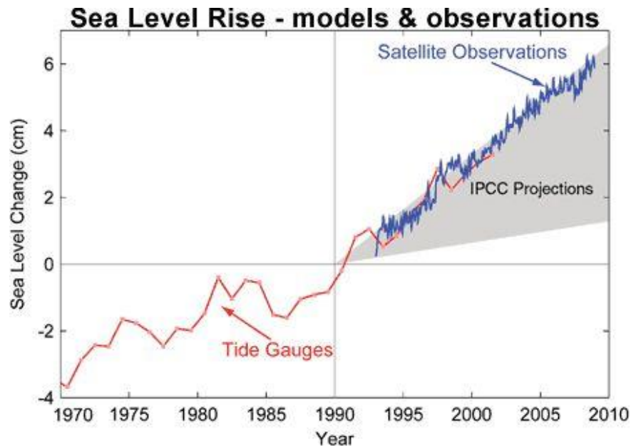
Figure 8.10: Observed sea-level rise, 1970-2010.
