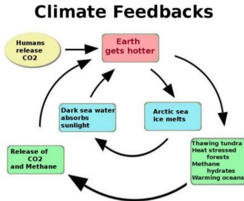
Figure 3.5: This diagram shows two important feedback loops, one involving the albedo effect, and the other involving methane hydrates.
