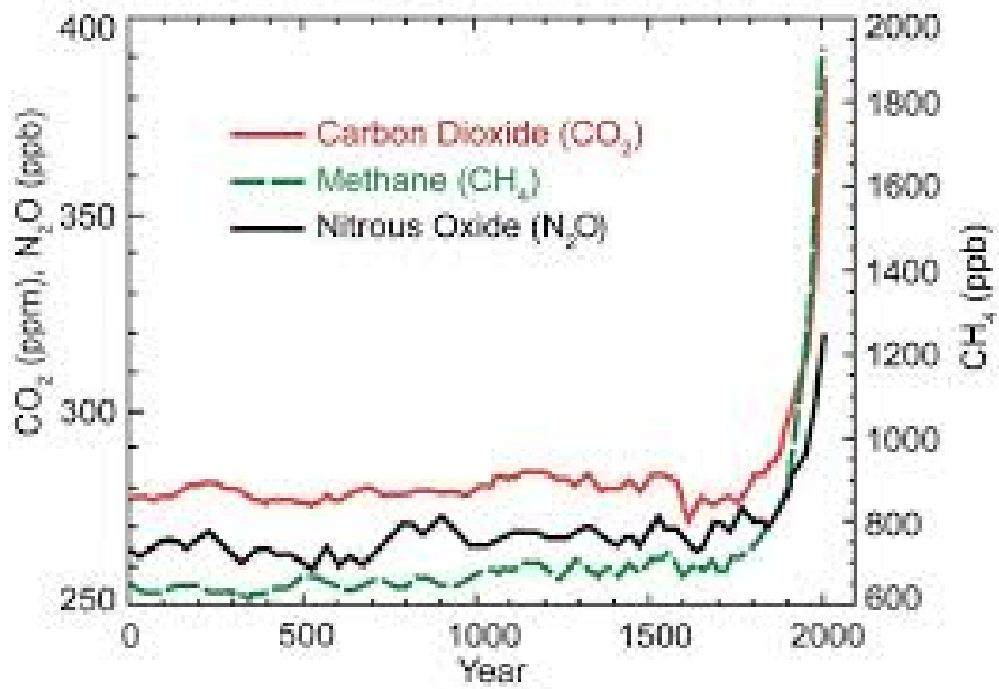
Figure 2.14: Concentrations of the most important greenhouse gases plotted as functions of time.
