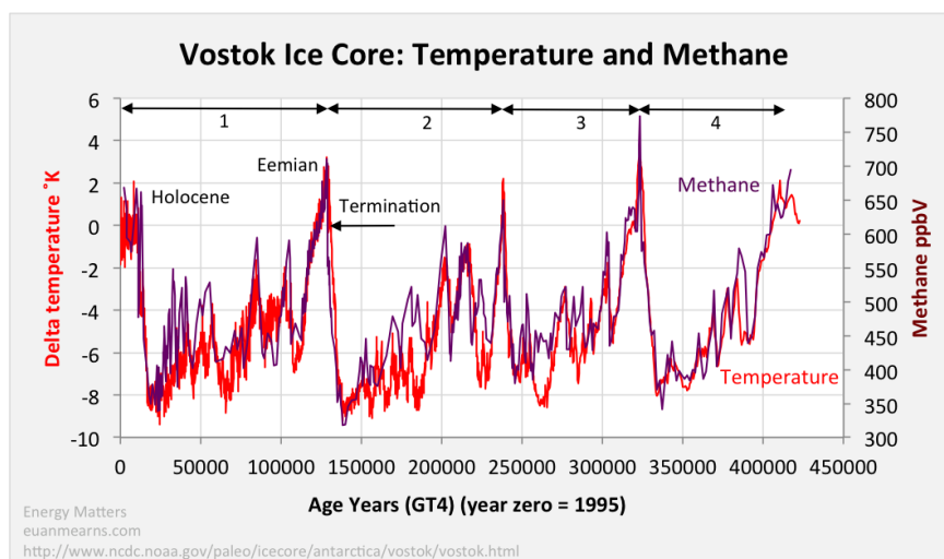
Figure 8.9: In ice core data, we see a close correlation between temperature and atmospheric CO 2 . There is also a close correlation between temperature and atmospheric methane.
