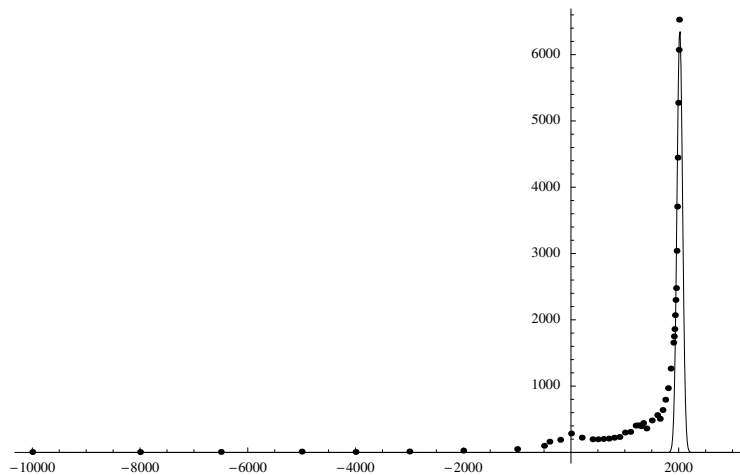
Figure 2.2: Population growth and fossil fuel use, seen on a time-scale of several thousand years. The dots are population estimates in millions from the US Census Bureau. Fossil fuel use appears as a spike-like curve, rising from almost nothing to a high value, and then falling again to almost nothing in the space of a few centuries. When the two curves are plotted together, the explosive rise of global population is seen to be simultaneous with, and perhaps partially driven by, the rise of fossil fuel use. This raises the question of whether the world's population is headed for a crash when the fossil fuel era has ended. (Author's own graph)
