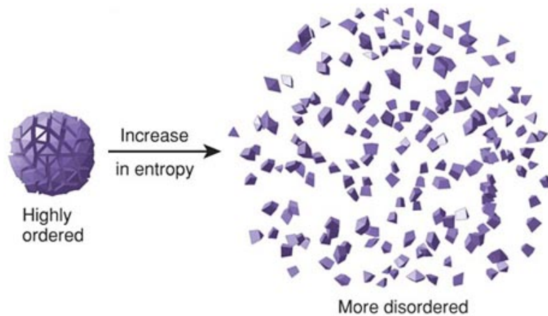
Figure 7.2: According to the second law of thermodynamics, the entropy of the universe constantly increases. Increase of entropy corresponds to increase of disorder, and also to increase of statistical probability. Living organisms on the earth are able to achieve a high degree of order and highly improbable structures because the earth is not a closed system. It constantly receives free energy (i.e. energy capable of doing work) from the sun, and this free energy can be thought of as carrying thermodynamic information, or “negative entropy”. Source: flowchainsensel.wordpress.co ,
