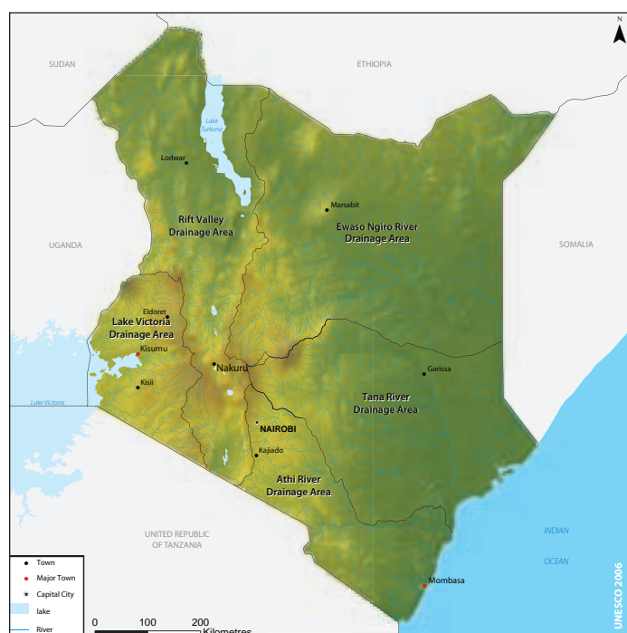
Figure 2: Kenya's surface drainage systems
