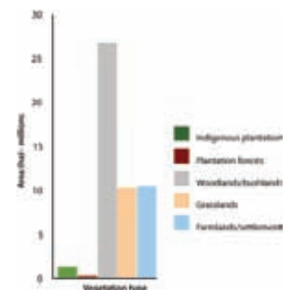
Figure 4: Land use area, 2005 (Source: KFS 2006)
