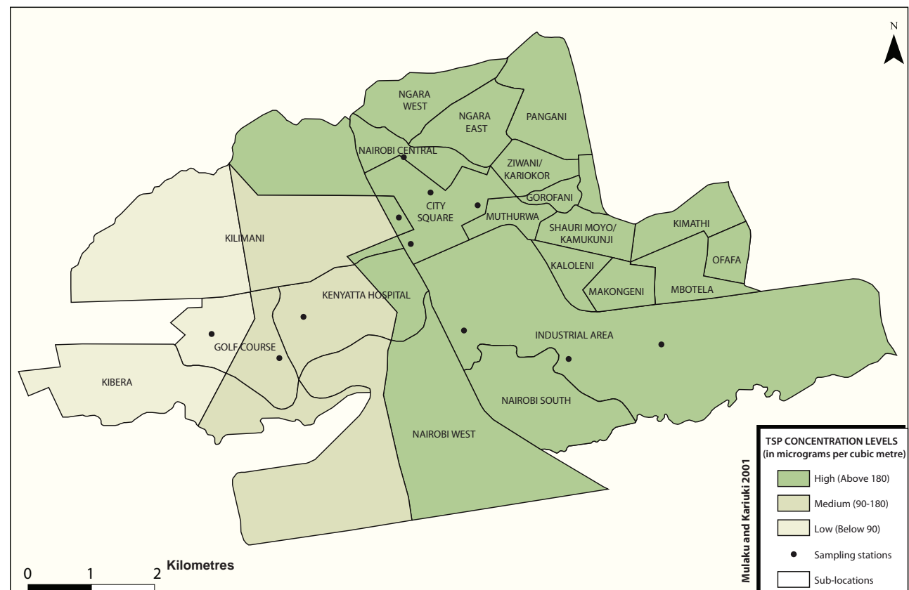
Figure 5: Average total suspended particulates (TSP) over a section of Nairobi
