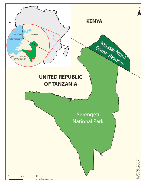
Figure 3: Location of Maasai Mara Game Reserve and Serengeti National Park
