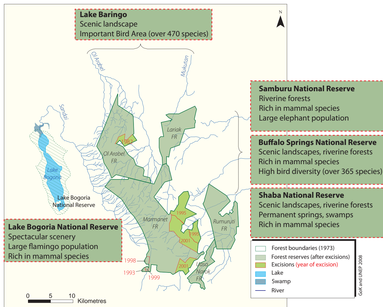
Figure 11: Marmaret forests are critical to major conservation areas
