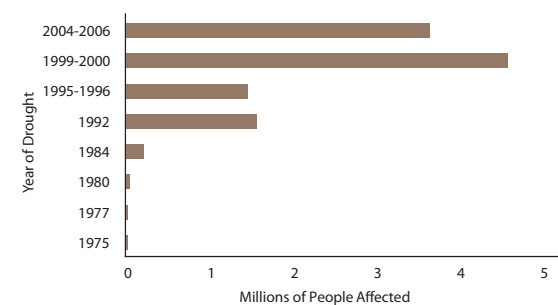
Figure 19: Number of Kenyans (million) affected by drought, 1975-2006 (Source: KMD 2008)
