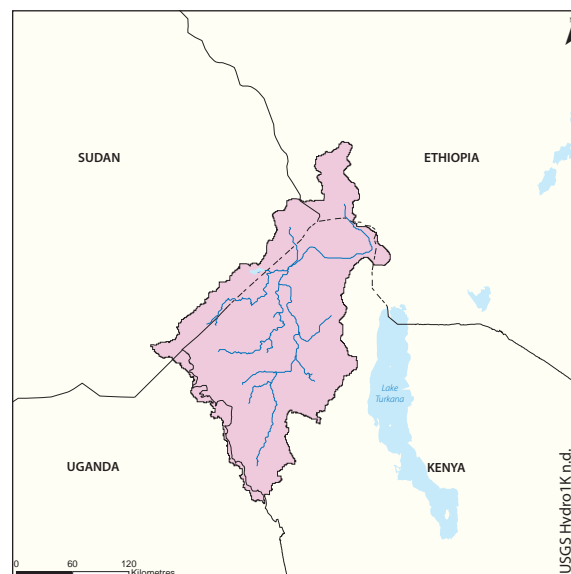
Figure 20: Location of Lotagipi Swamp
