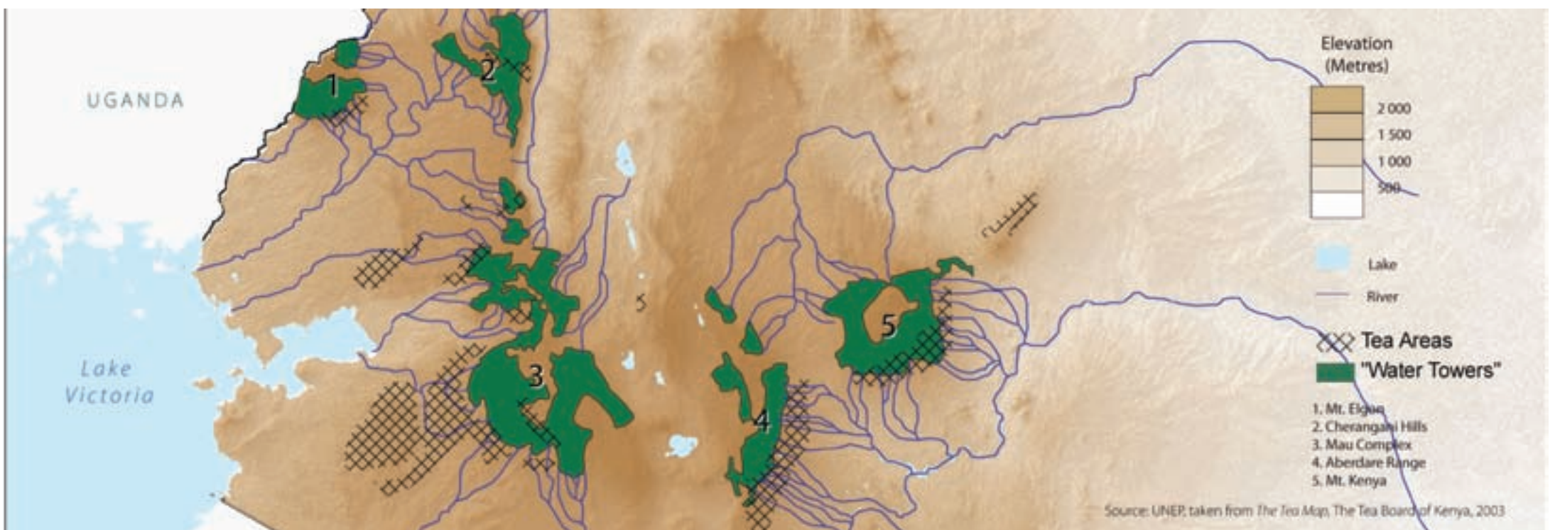
Figure 8: Kenya's tea growing areas and the five "water towers" (Source: UNEP, taken from The Tea Map, The Tea Board of Kenya, 2003)
