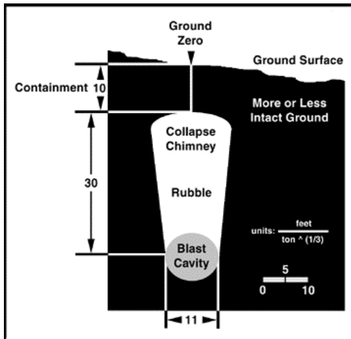
Figure 3 Schematic Diagram of Blast Cavity and Collapse Chimney
