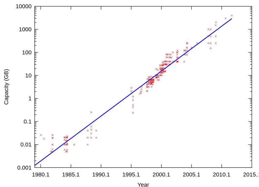
Figure 15.18: A logarithmic plot of the increase in PC hard-drive capacity in gigabytes. An extrapolation of the rate of increase predicts that the individual capacity of a commercially available PC will reach 10,000 gigabytes by 2015, i.e. 10,000,000,000,000 bytes. (After Hankwang and Rentar, Wikimedia Commons)
