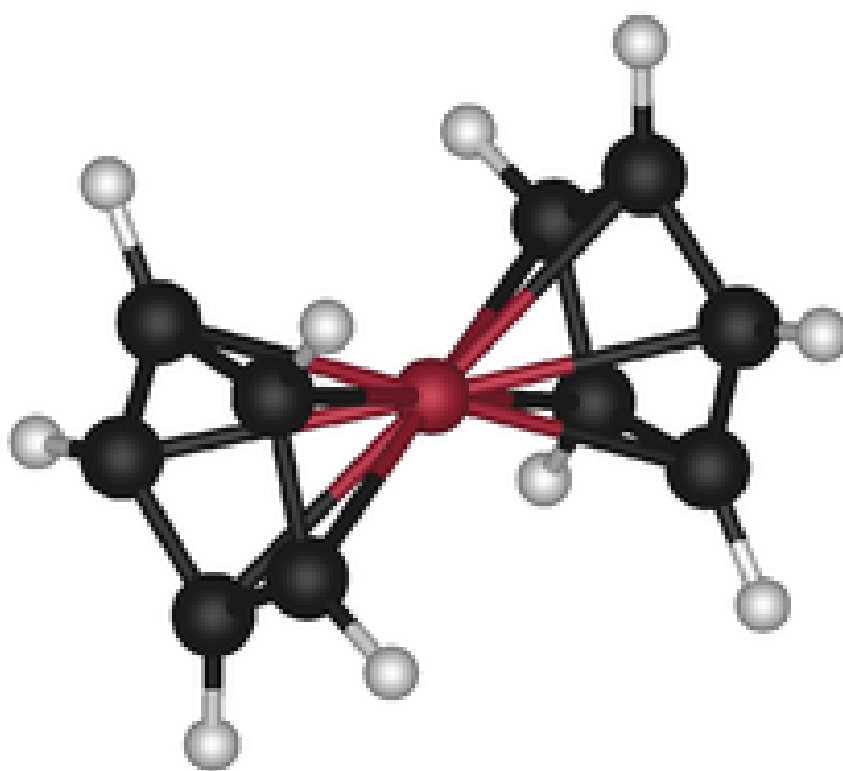
Figure 13.3: The structure of ferrocene \text{Fe}(\text{C}_5\text{H}_5)_2 .
