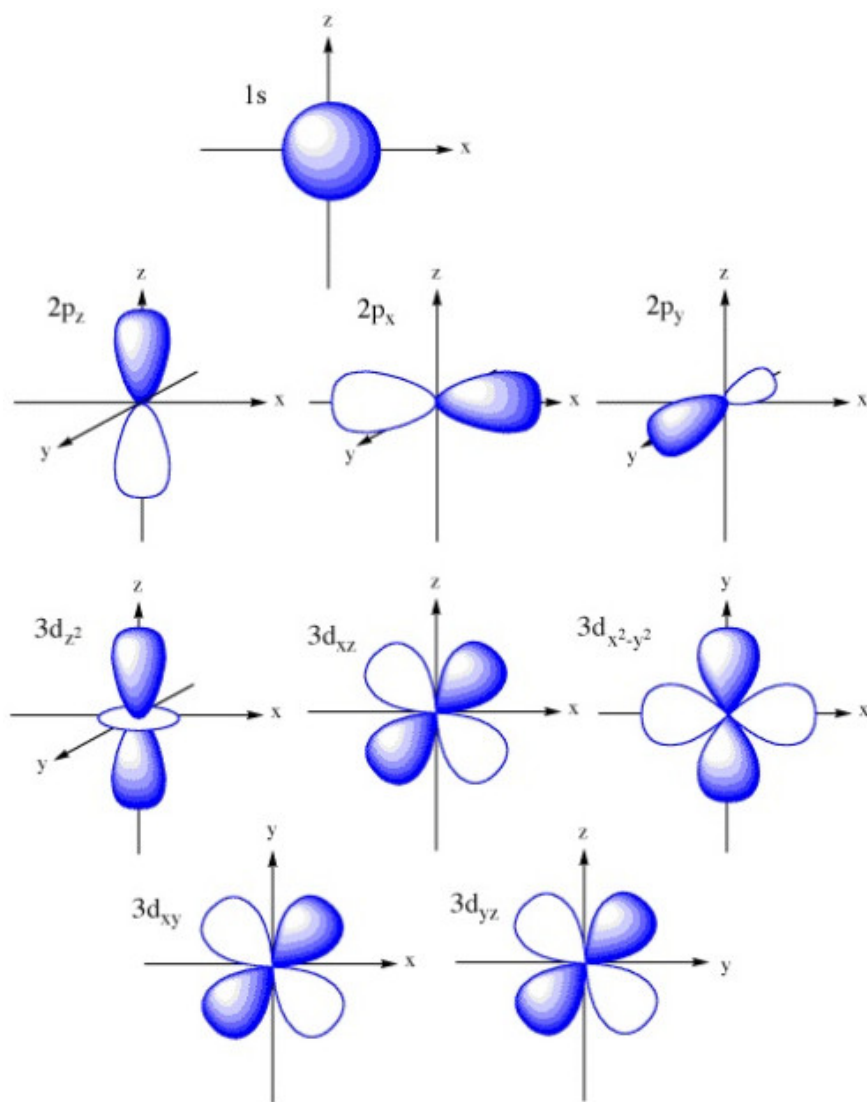
Figure 11.6: Atomic orbitals.
