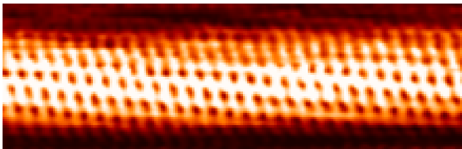
Figure 16.10: An STM image of a single-walled carbon nanotube.
